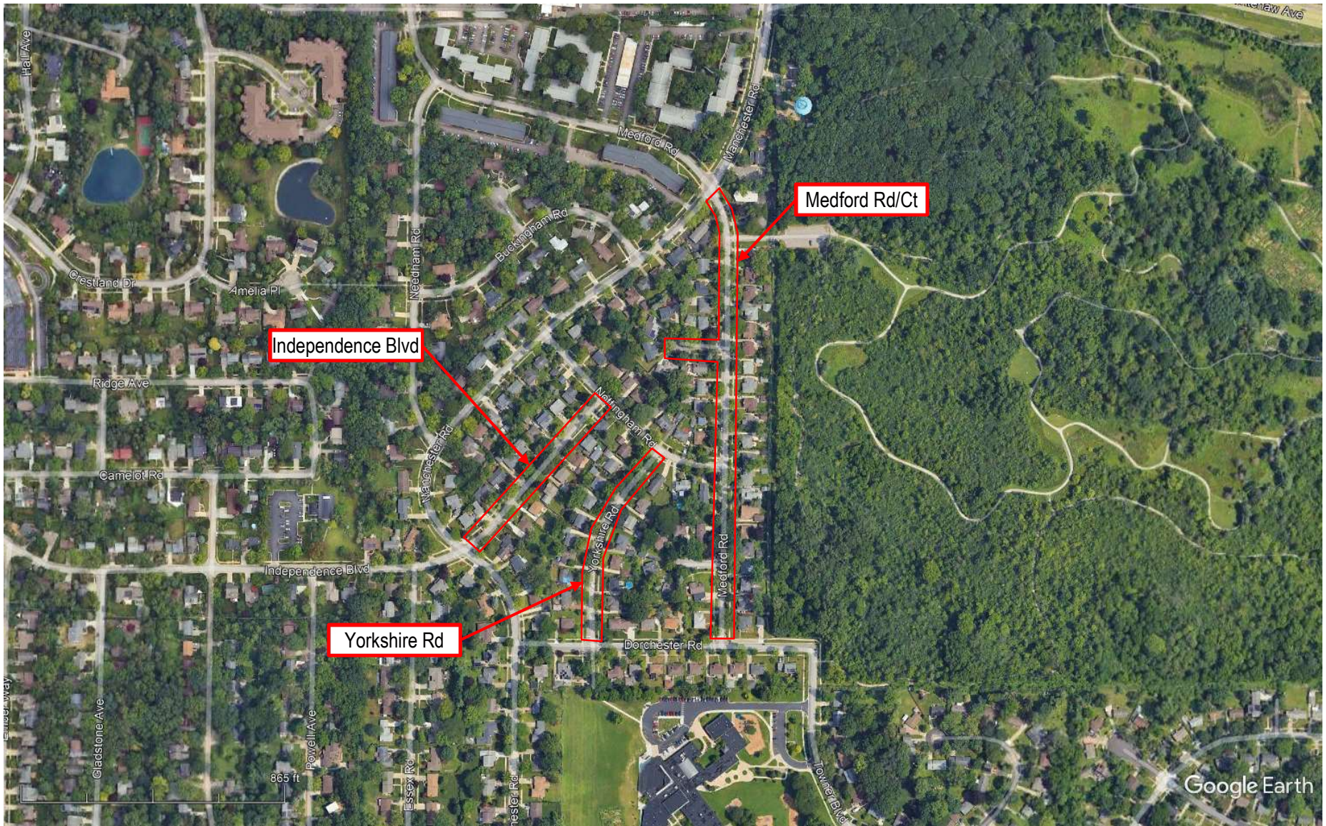
Figure 1: Site Location Map (Independence Blvd, Yorkshire Rd, Medford Rd/Ct) 2023 Bundle 2 – Water Main Replacement Independence Blvd, Yorkshire Rd, Medford Rd/Ct, Ann Arbor, Michigan MSG Project Number: 401.2300021.000
